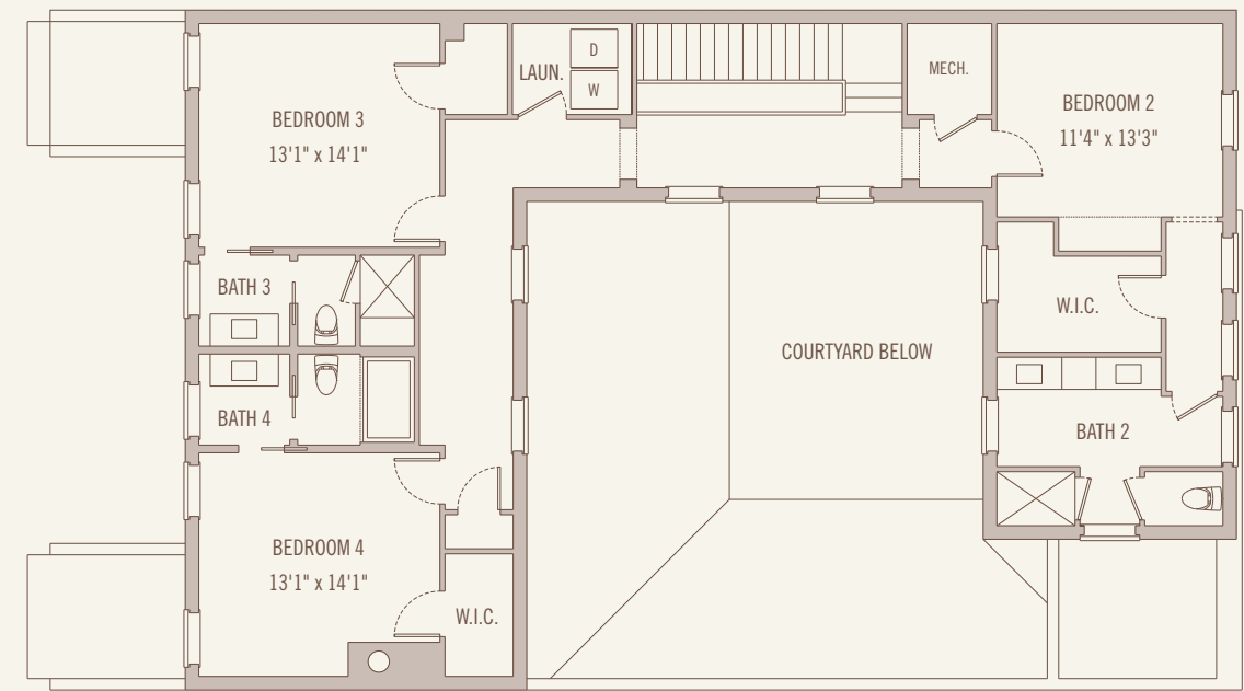
SECOND FLOOR AA - 2
