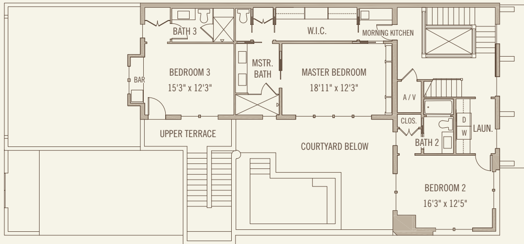
SECOND FLOOR Z-1
