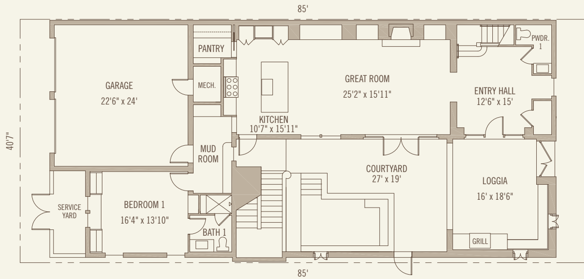
FIRST FLOOR Z-1
