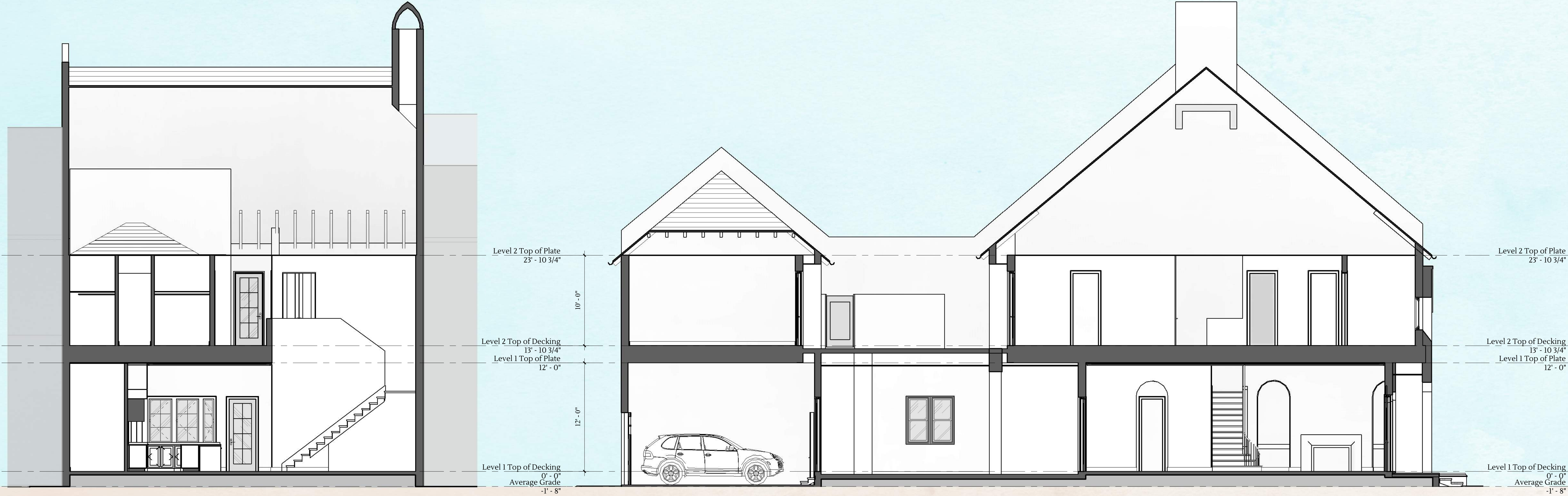
TRANSVERSE SECTION
