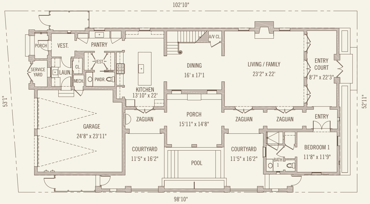
FIRST FLOOR CC - 14
