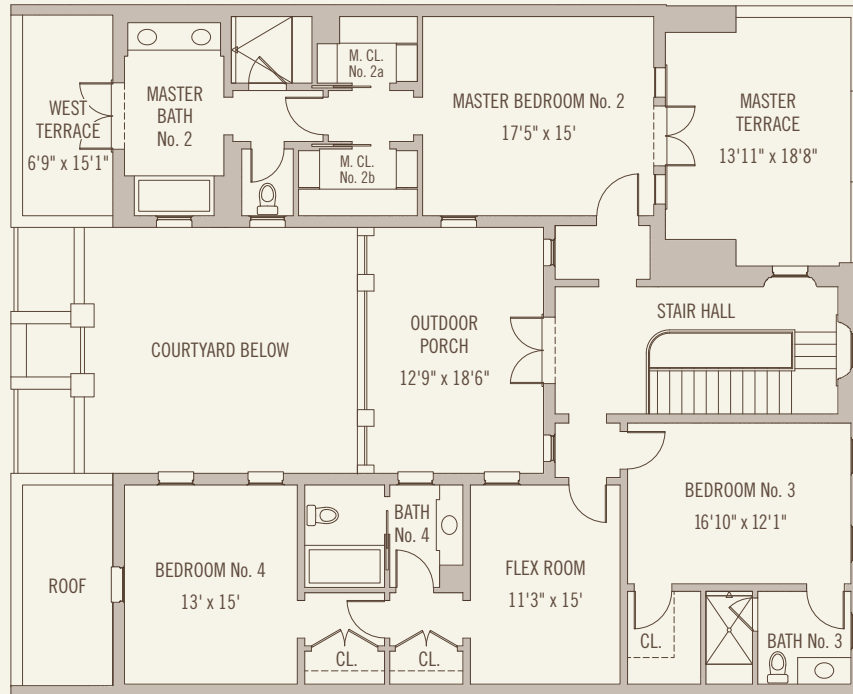
SECOND FLOOR BB - 5
