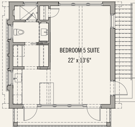
SECOND FLOOR GARAGE
