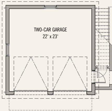
FIRST FLOOR GARAGE
