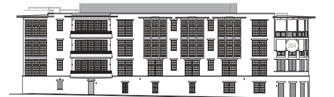
WEST ELEVATION
