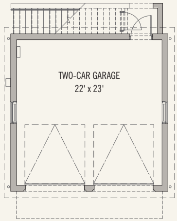
FIRST FLOOR GARAGE
